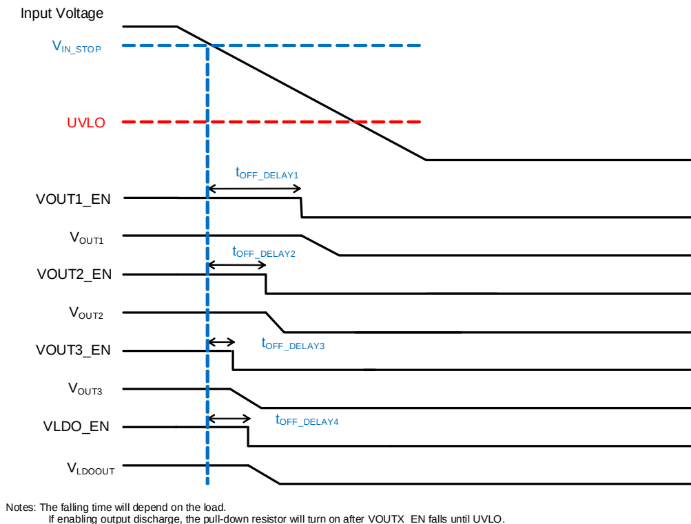
Figure 4: Power-Off Sequence
