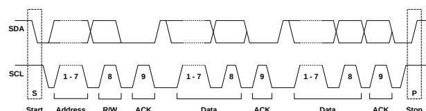
Figure 11: A Complete Data Transfer
