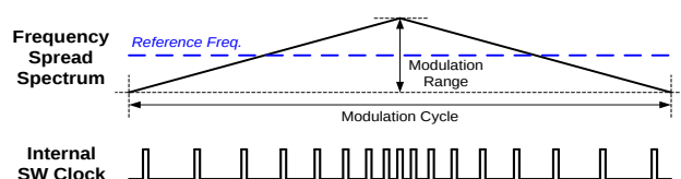
Figure 5: Frequency Spread Spectrum
