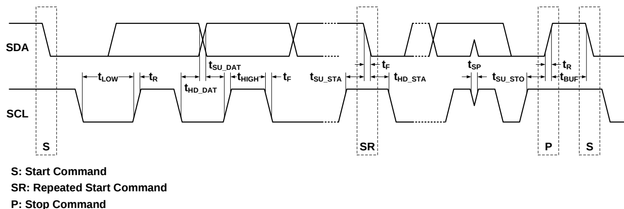
Figure 1: I 2 C-Compatible Interface Timing Diagram
