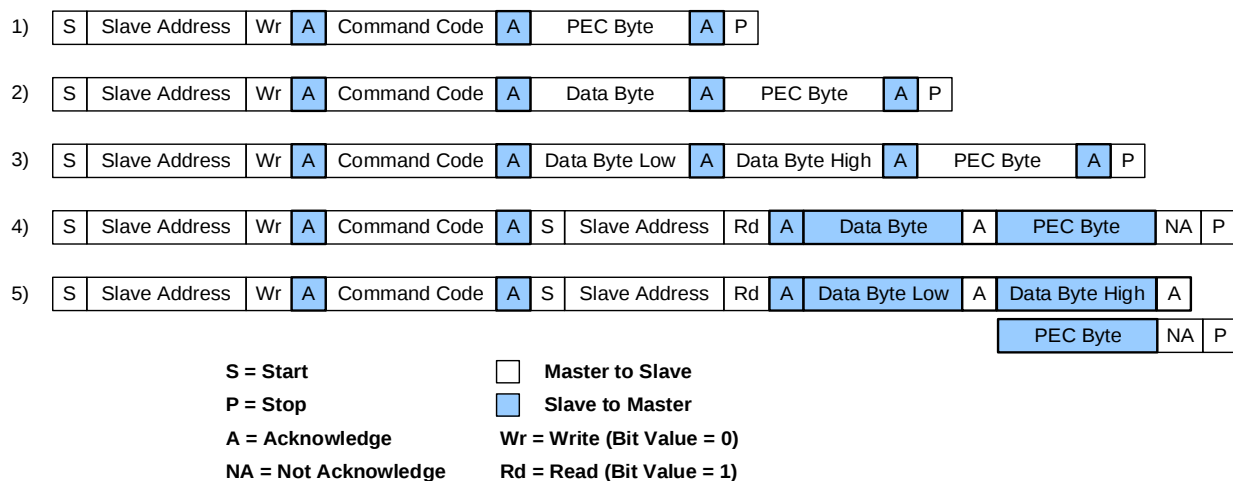
Figure 13: I²C Write/Read Sequence with PEC
