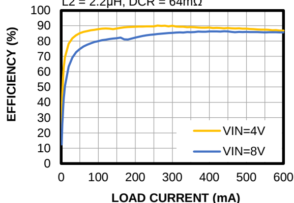
Efficiency vs. Load Current (Buck 3)
