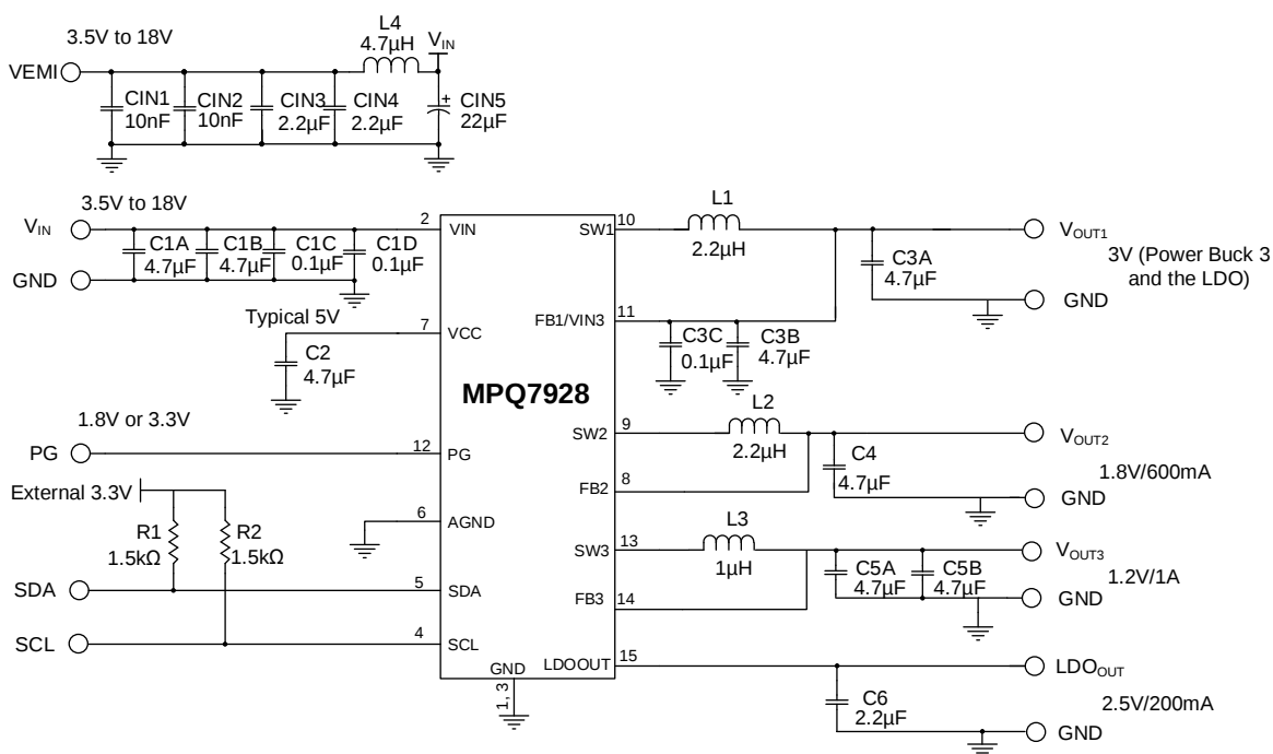
Figure 17: Typical Application Circuit ( V_{OUT1} = 3V , V_{OUT2} = 1.8V , V_{OUT3} = 1.2V , V_{LDO} = 2.5V with EMI Filters)
