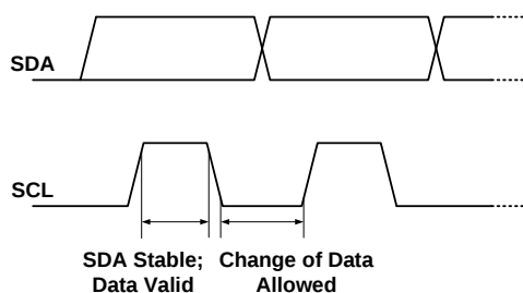
Figure 9: Bit Transfer
