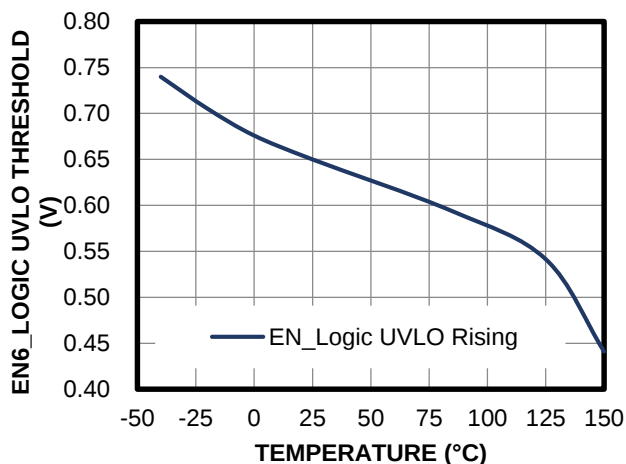
EN6_Logic UVLO Threshold vs. Temperature
