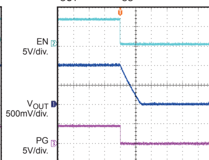
Power Good through EN Shutdown
