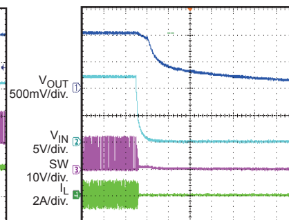
Shutdown Through VIN
