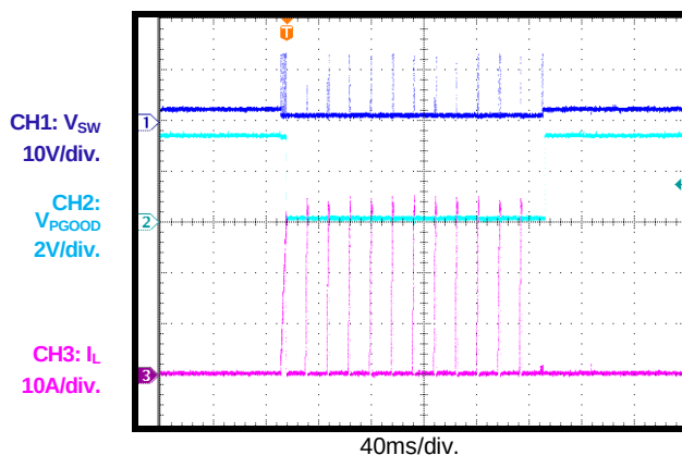
OCP, Hiccup Option, DCM, Single-Phase
