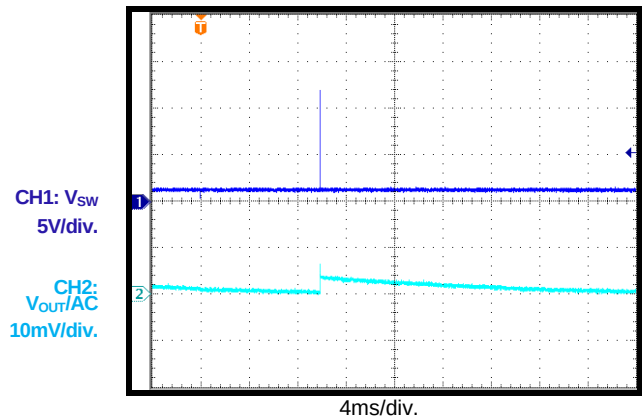
I_{OUT} = 0A , DCM, 1000kHz, Single-Phase
