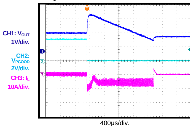
OVP, Latch-Off Option, CCM, Single-Phase
