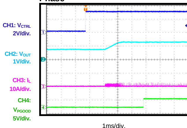
Pre-Bias Start-Up, DCM, Single-Phase
