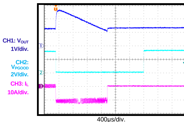
OVP, Hiccup Option, CCM, Single-Phase
