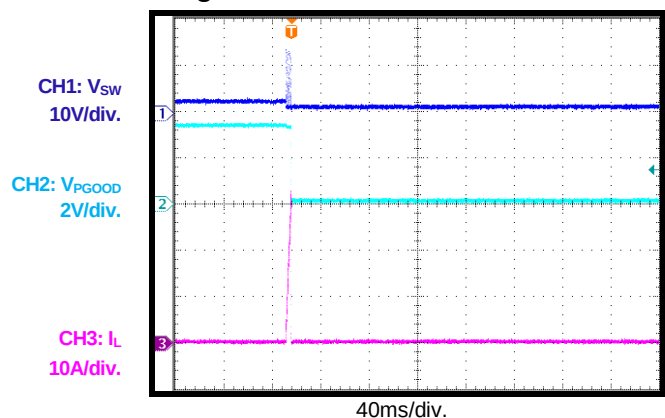
OCP, Latch-Off Option, DCM, Single-Phase
