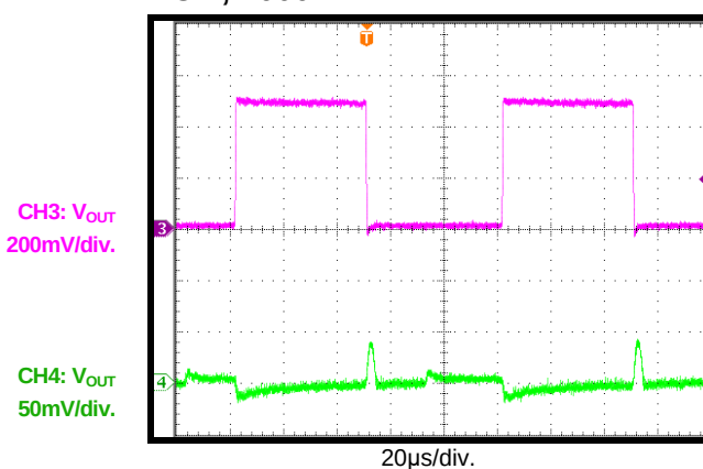
Load Transient, I_{OUT} = 0A to 10A , DCM, 1000kHz
