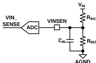
Figure 14: V_{IN} Sensing Block Diagram
