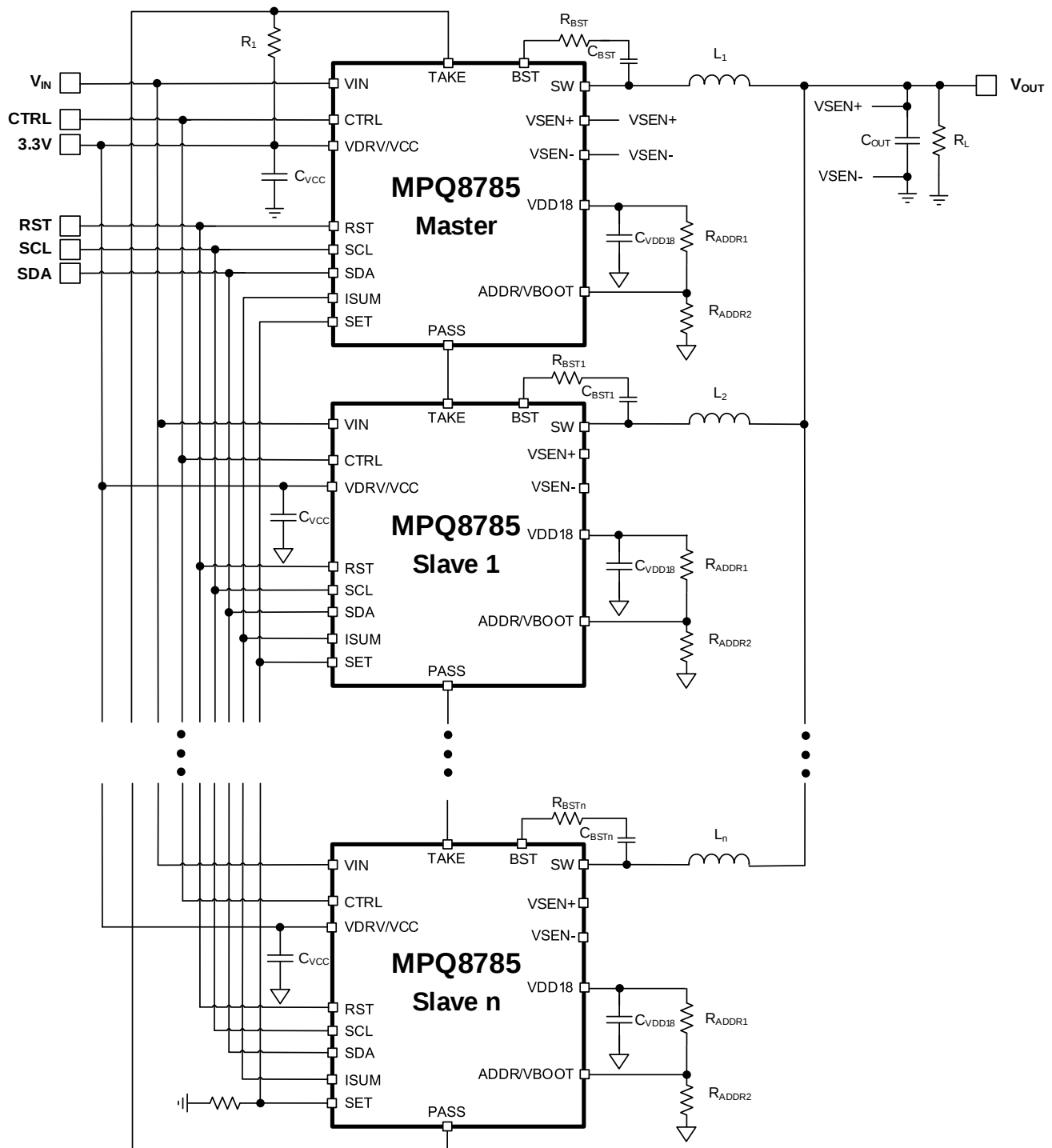
Figure 3: Multi-Phase Operation
