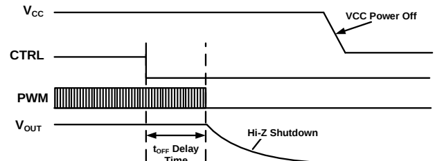
Figure 10: Shutdown Sequence with Hi-Z Shutdown
