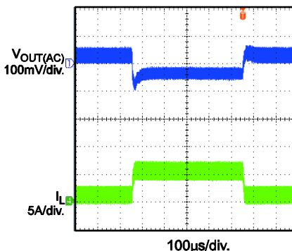
Transient I_{OUT}=0.6A-5.4A@2.5A/\mu s , F_{SW}=500kHz , C_{OUT}=3 \times 22\mu F
