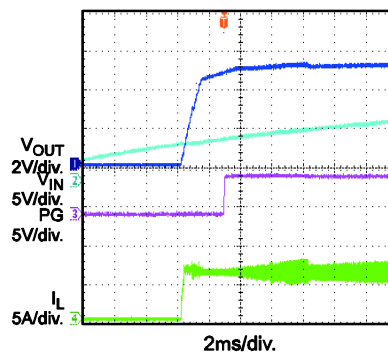
Power Good Through Vin Start-Up I_{OUT}=6A
