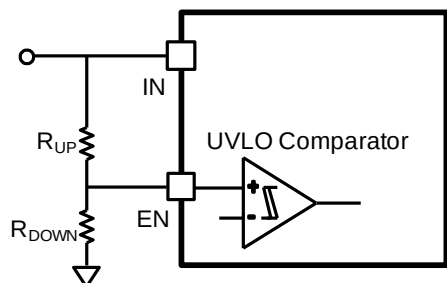
Figure 8—Adjustable UVLO
