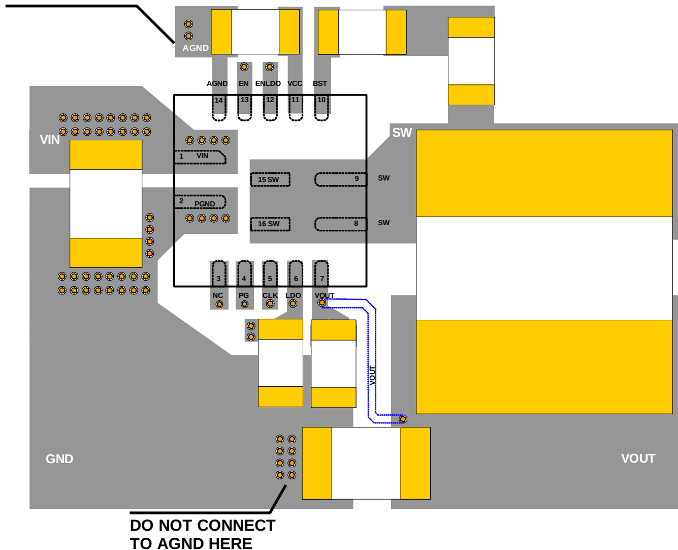
Figure 9—Recommend Layout
