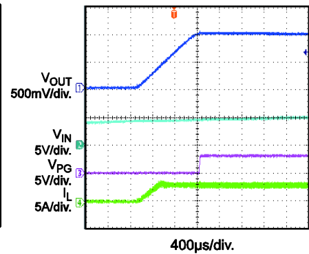
Power Good through VIN Start-Up I_{OUT} = 3A
