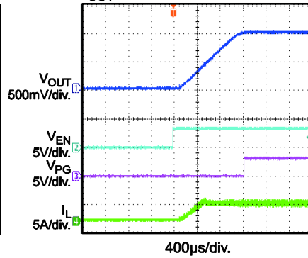
Power Good through EN Start-Up I_{OUT} = 3A
