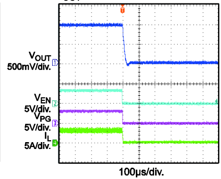
Power Good through EN Shutdown I_{OUT} = 3A
