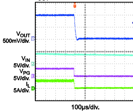
Power Good through VIN Shutdown I_{OUT} = 3A
